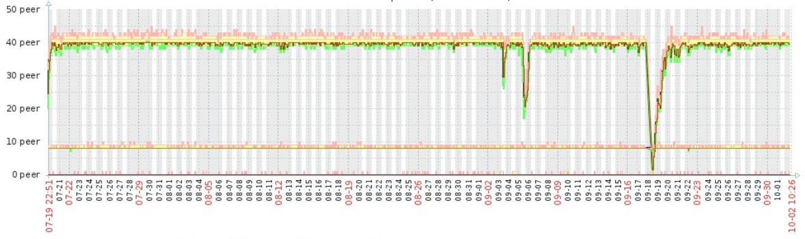
docker: Vertcoind peers (2m 14d 11h)
