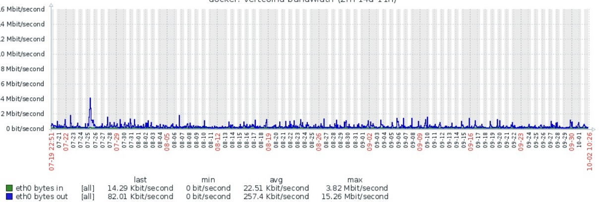
docker: Vertcoin bandwidth (2m 14d 11h)
